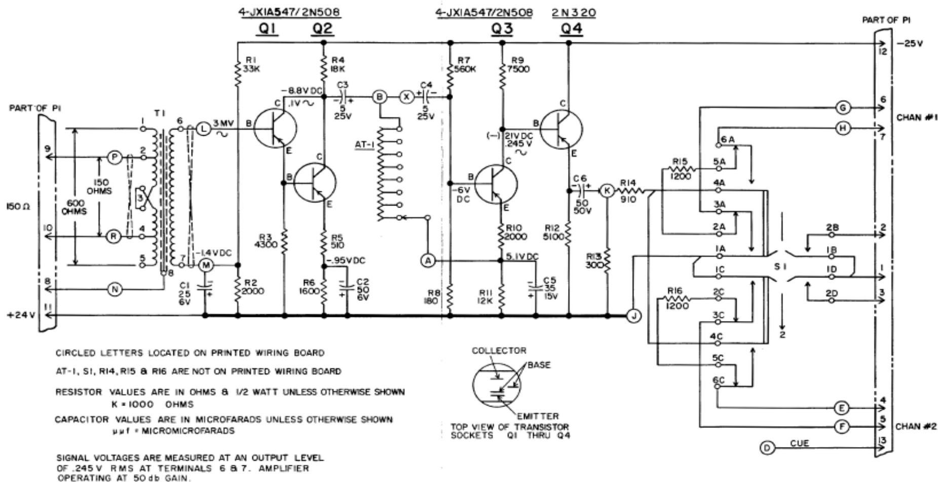
Fig. 5 Elementary Diagram, Pre-Amplifier, Model 4BA21A1 (C-7777444, Rev. A)
